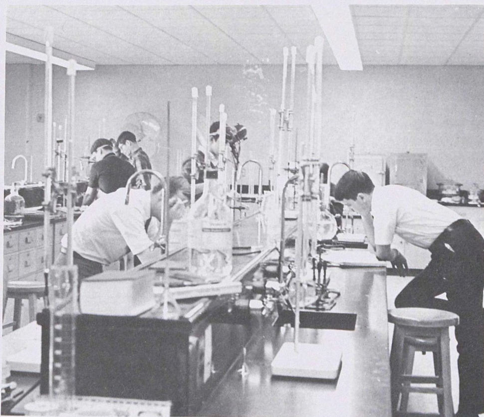
Students calculate titrations
